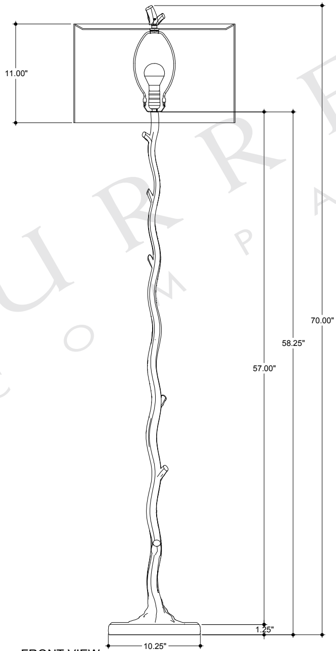
FRONT VIEW
